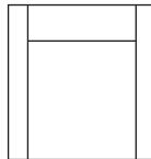
40510 | CHAIR TOTAL | W37" D35" H34" SEAT | W25" D22" H20" ARMS | --- --- h26"
